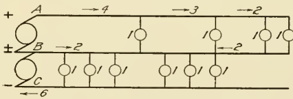
Fig. 12. Diagram of 3-Wire System—Unbalanced Load
